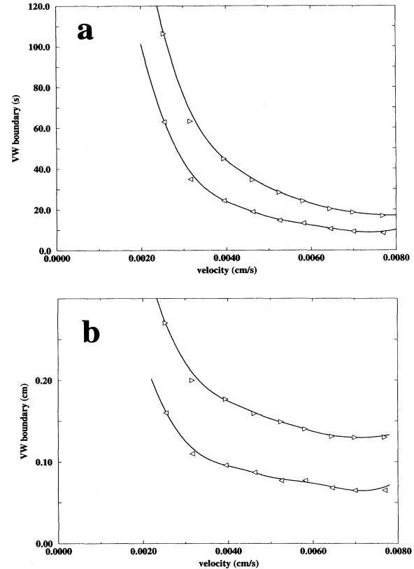
FIG. 3. Left boundary (upward triangles) and right boundary (downward triangles) of the VW measure in (a) time units and (b) space units as functions of the reference wave velocity.
